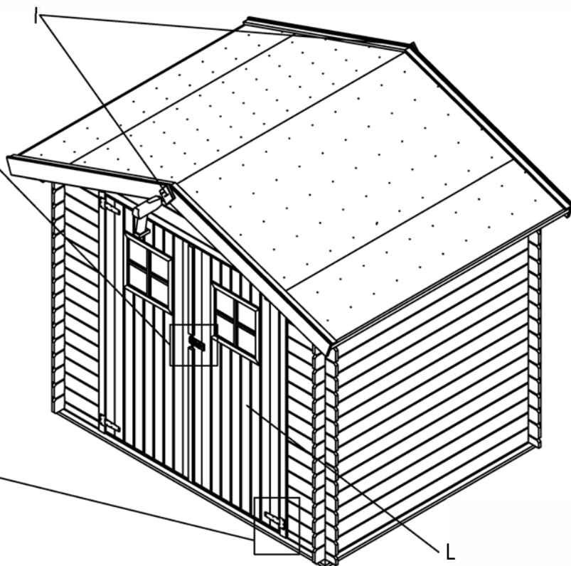
hinges - 4pcs screws 3x40mm - 40pcs
